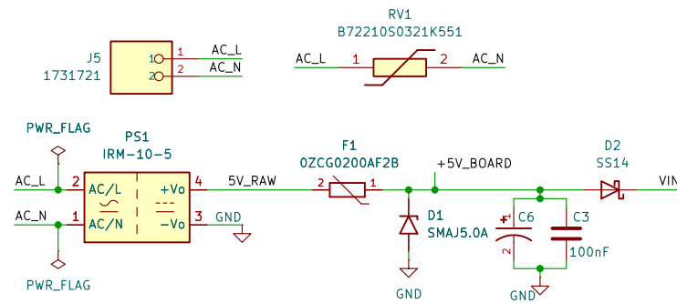
AC Power Input & Protection
