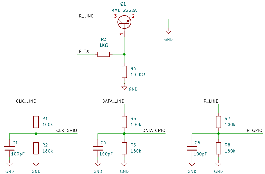
Signal Interface (Passive Taps & IR Driver)
