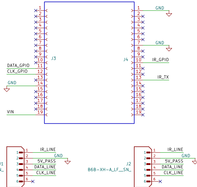
ESP32 DevKit Interface & JST Pass-Through Connectors
